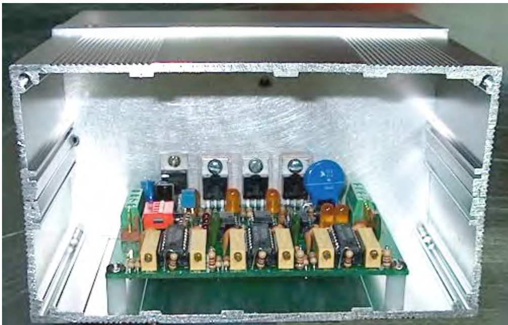
PWM3f board in aluminum extruded box.
